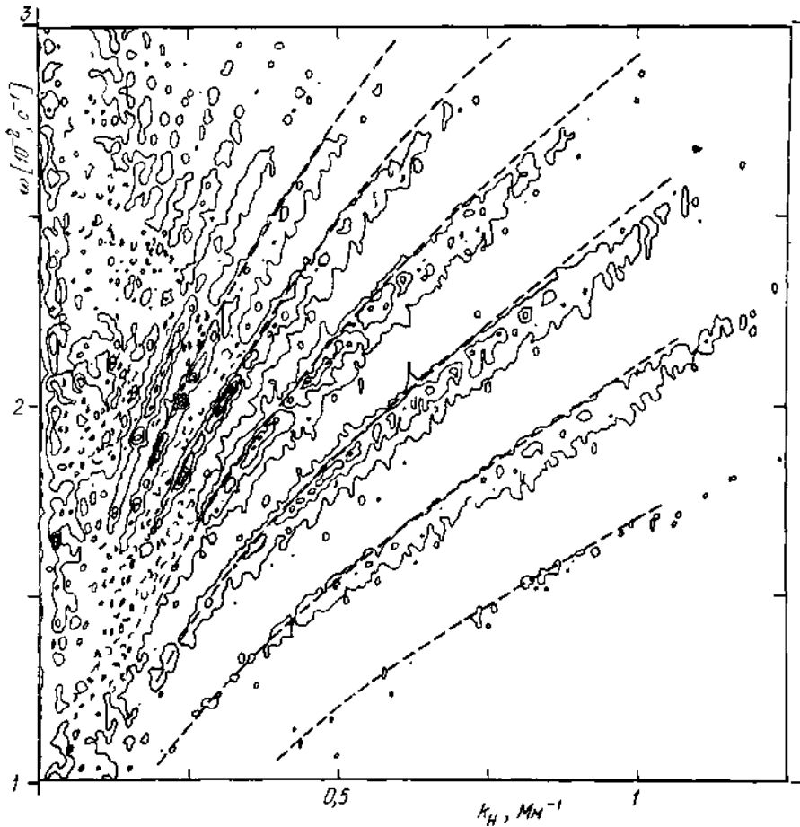
Fig. 1. Power spectrum of 5-minute oscillations in coordinates k_H, \omega .
