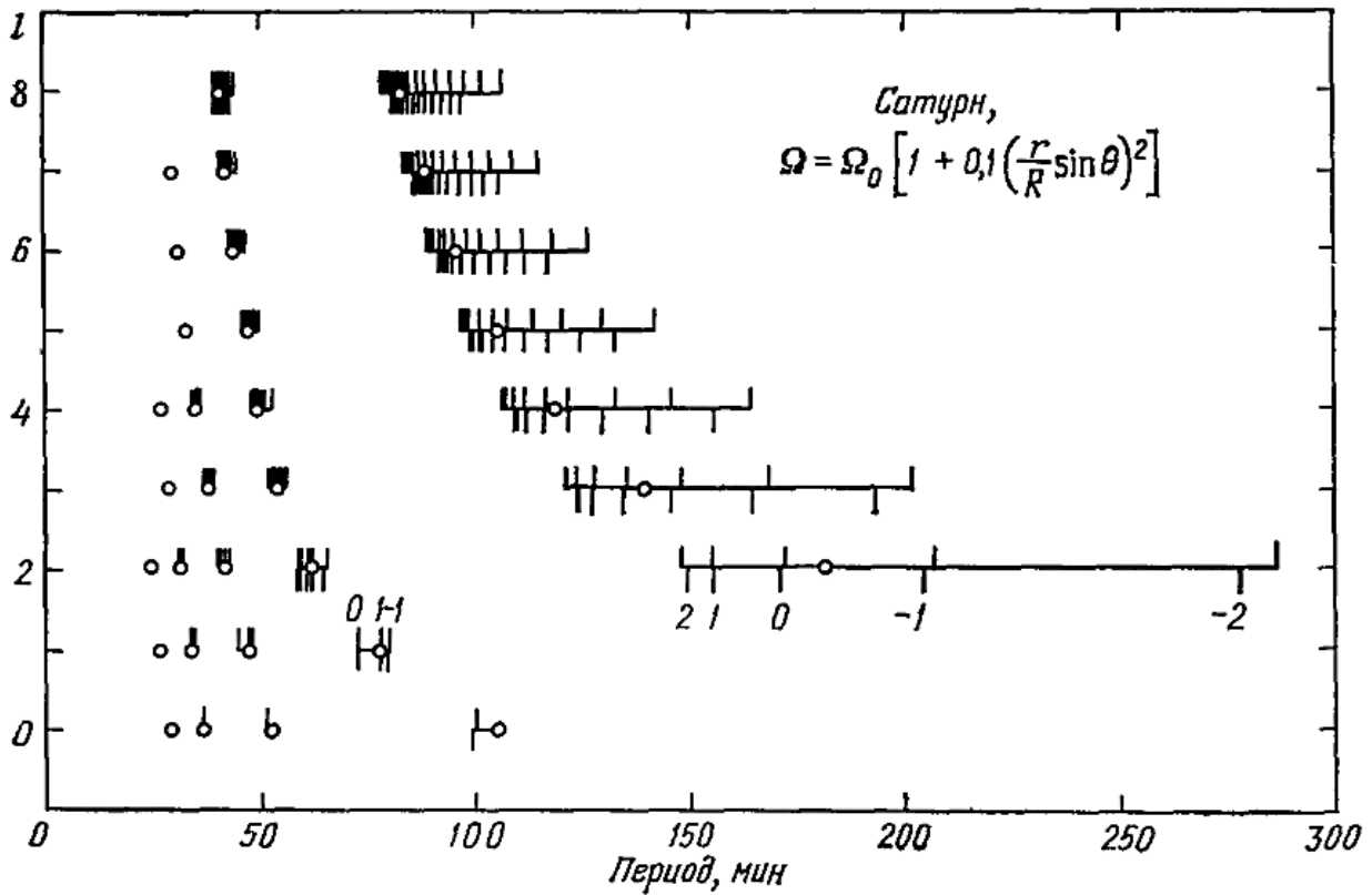
Fig. 2. Spectrum of Saturn's natural oscillations
