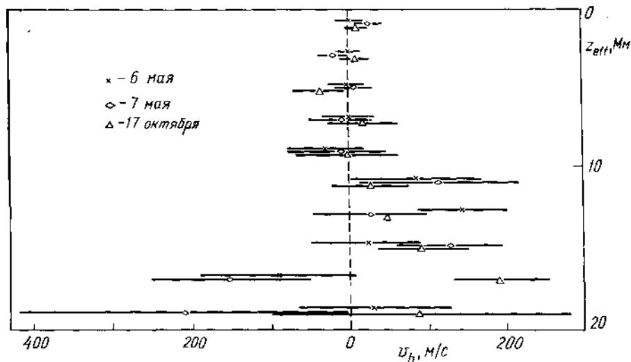
Fig. 2. Relative rotation speeds at the equator depending on the depth under photosphere.
