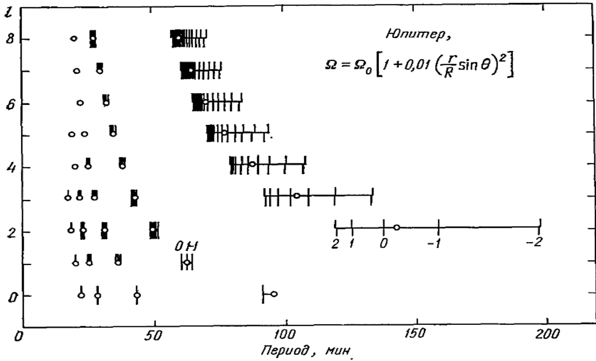
Fig. 1. Spectrum of Jupiter's natural oscillations
